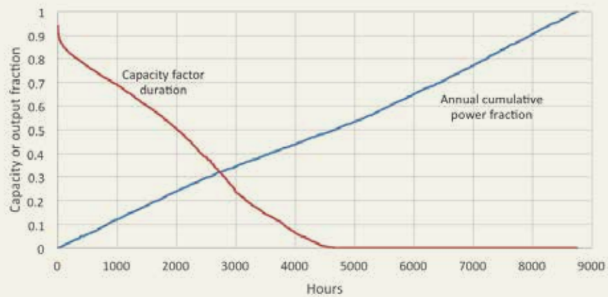
Figure 35: Combined system PV power performance indicators. Capacity factor duration curve (as a fraction by ranked hour) and annual cumulative power output (as a fraction by year hour).
