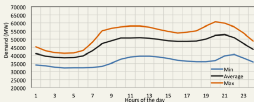
Figure 14: Minimum, average and maximum hourly demand based on the IRP Update Base Case scenario for 2030.
