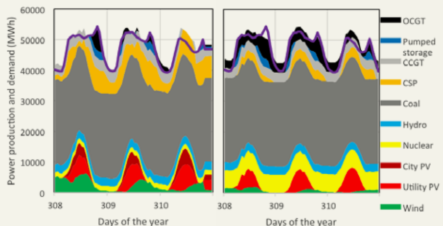
Figure 54: Comparison between WWF High (left) and IRP Update (right) for an early summer event demonstrating the importance of technology capacity balancing.
