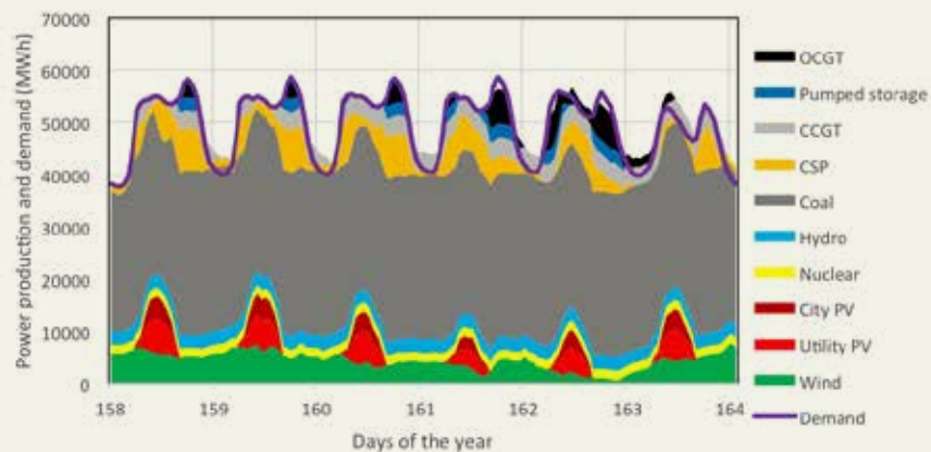
Figure 32: Winter week illustrating CSP in non-forecasting role: WWF High scenario.
