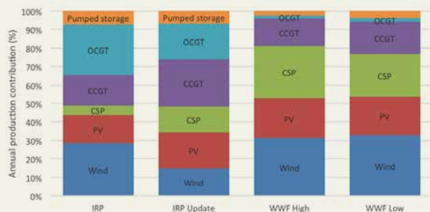
Figure 56: Annual electricity production balance for renewable, mid-merit and peaking for all 2030 scenarios.
