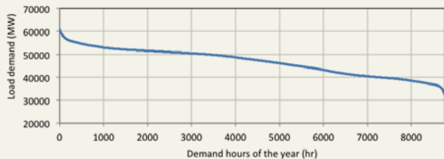
Figure 15: System demand duration curve. Based on the IRP Update Base Case Scenario for 2030.
