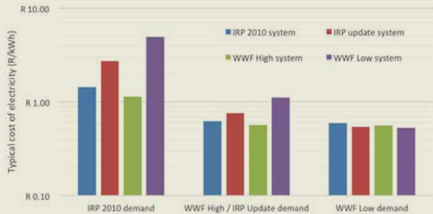
Figure 3: Cost probabilities of the scenarios using simple LCOE and 50 th percentile cost values.
